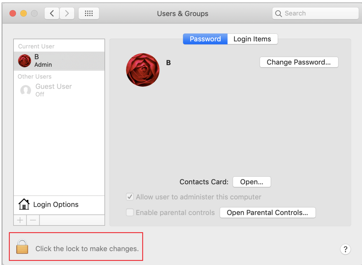
Figure 4. Users & Groups
